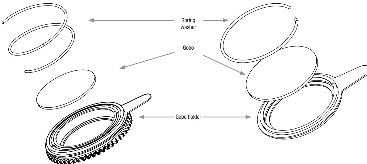
Gobo holder for rotating gobos
